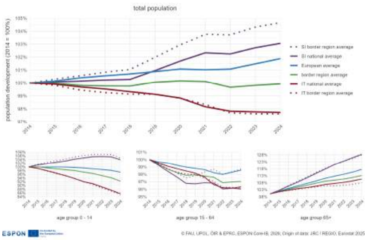
Figure 2.2: Population development (2014=100)
