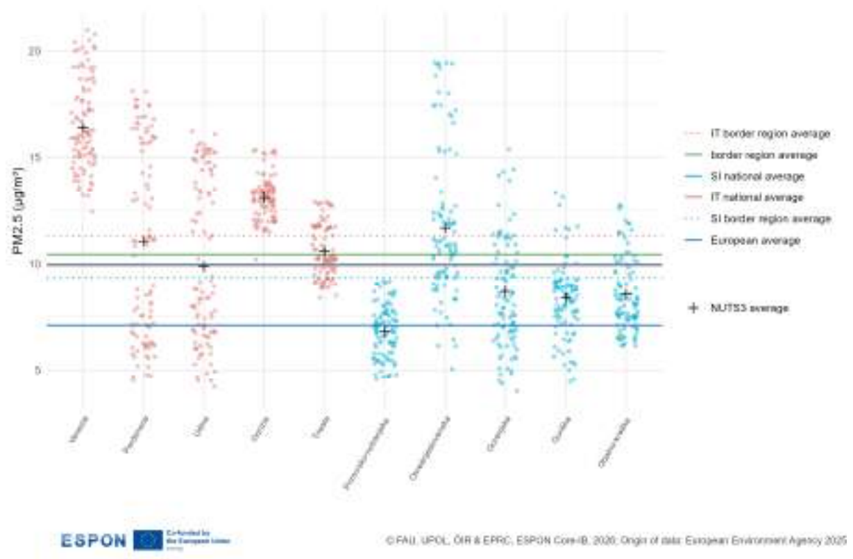
Figure 2.20: Air pollution
