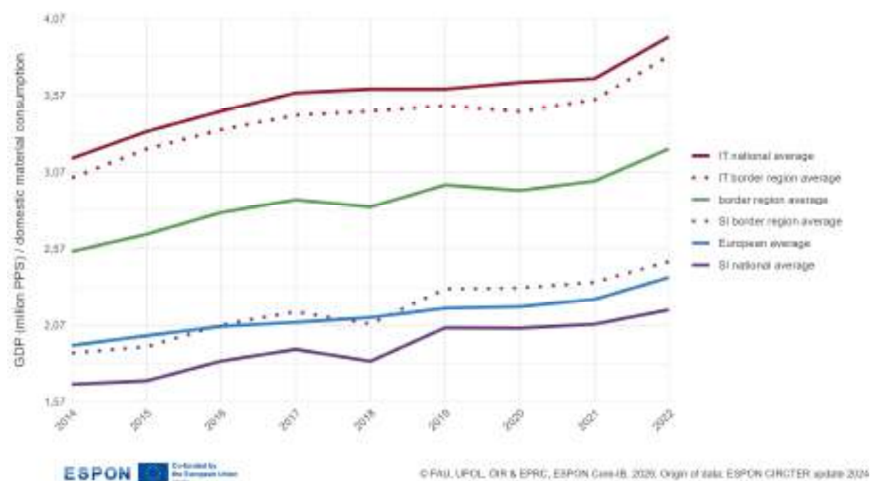
Figure 2.25: Resource productivity
